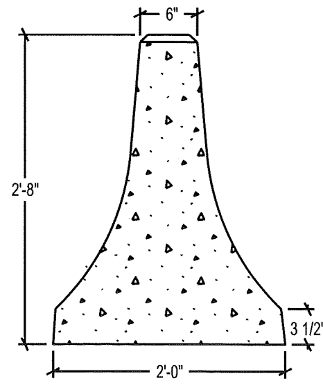
ELEVATION VIEW JERSEY BARRIER
