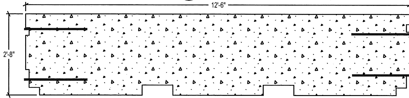
ELEVATION VIEW JERSEY BARRIER
