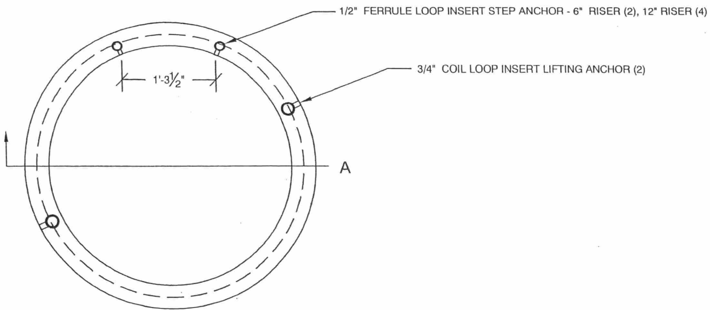
PLAN
