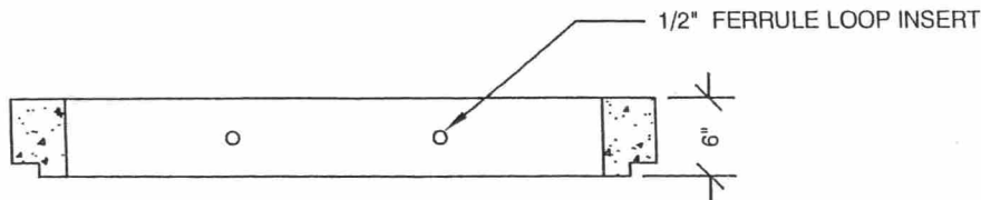
SECTION A - 6" RISERS AND 12" RISERS
