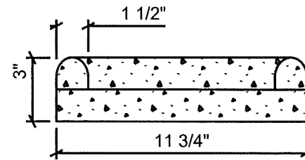
END VIEW 12"X24" SPALSH BLOCK
