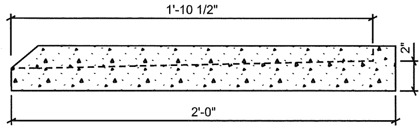
SIDE VIEW 12"X24" SPALSH BLOCK
