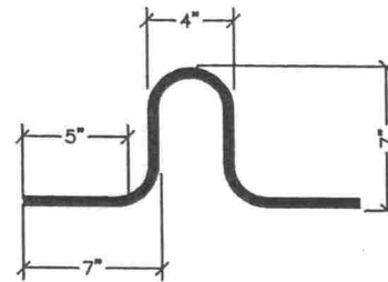
(C) GALV. LIFTING LOOP DETAIL
