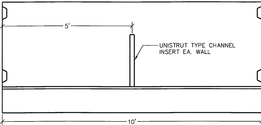
SIDE VIEW 10' UTILIDOR SECTION
