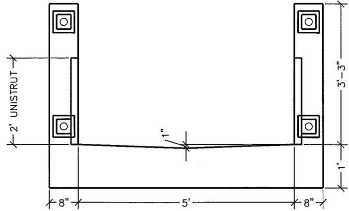
END VIEW 10' UTILIDOR SECTION
