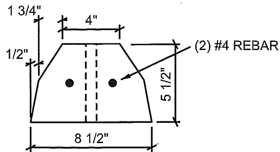
CUT VIEW 6' WHEELSTOP A -
