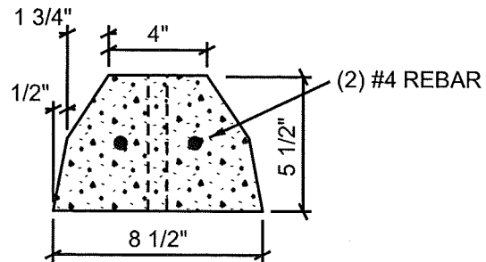
CUT VIEW 6' WHEELSTOP
