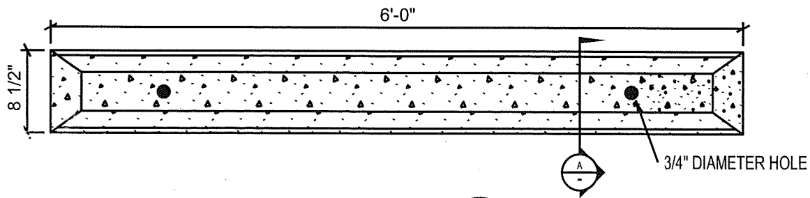
PLAN VIEW 6' WHEELSTOP
