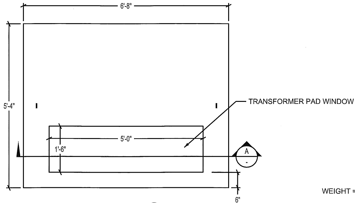
PLAN VIEW GVEA KVA 1500
