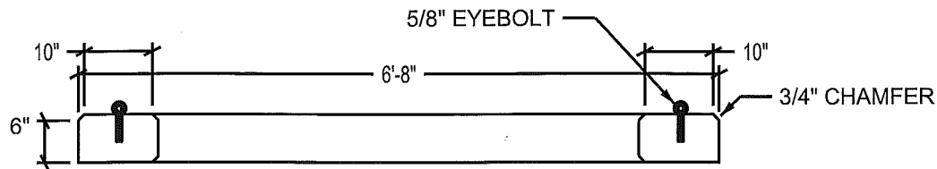
SECTION THROUGH OPENING GVEA KVA 1500
