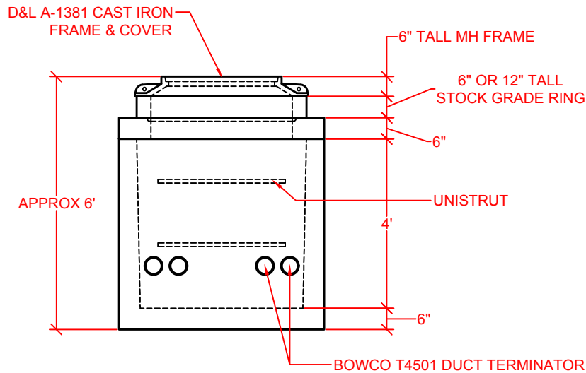
TYPICAL STACKED ELEVATION
