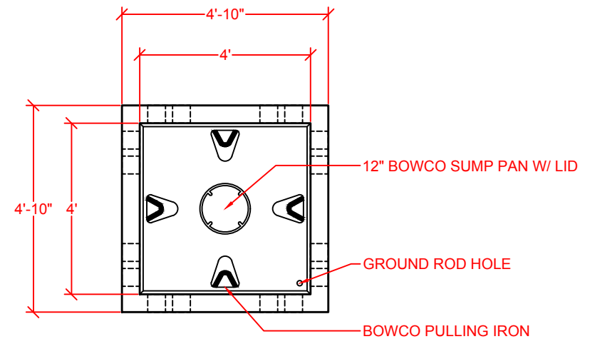
VAULT BASE: PLAN
