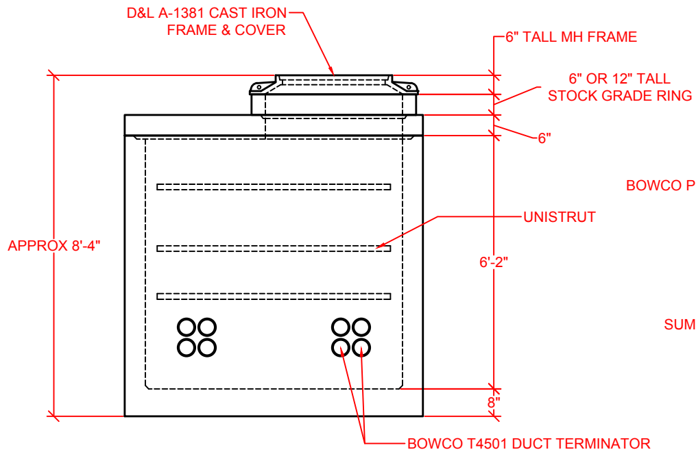
LONG WALL STACKED ELEVATION
