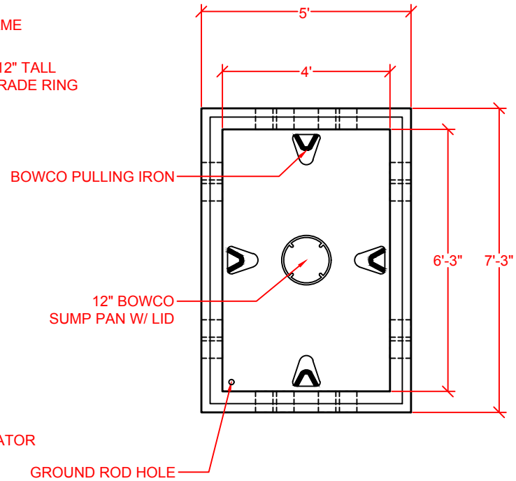
VAULT BASE: PLAN
