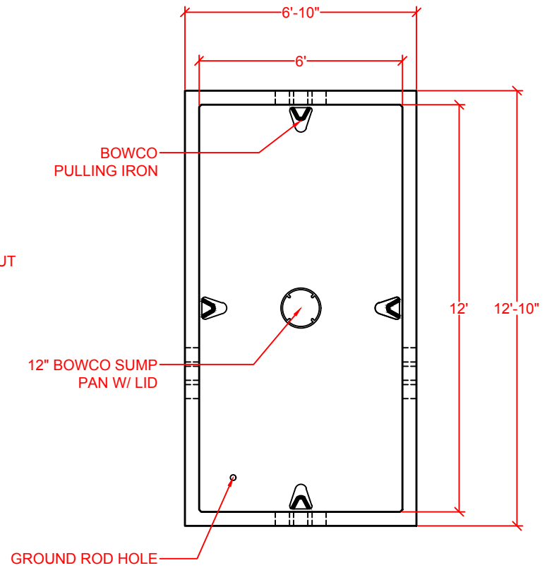
VAULT BASE: PLAN
