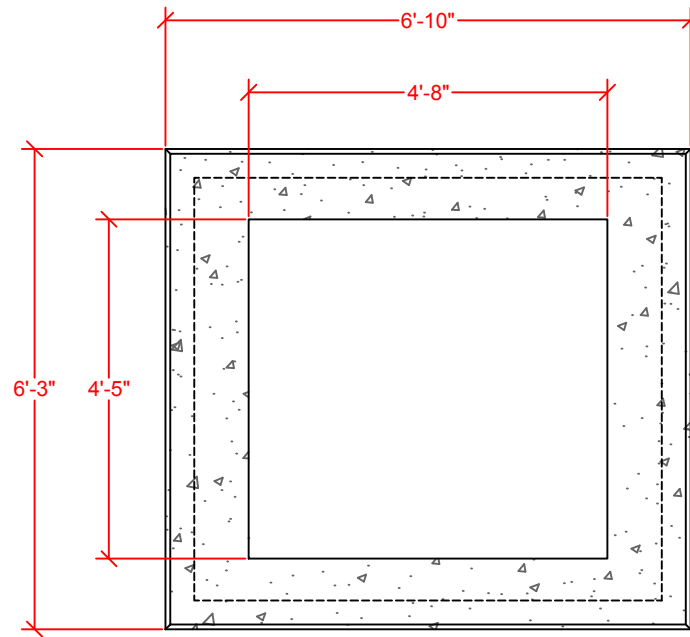
PLAN VIEW
