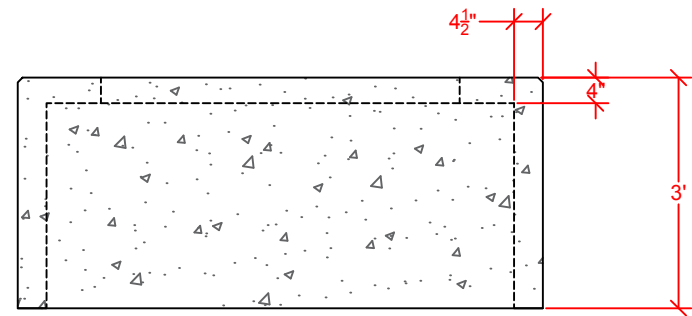
PROFILE VIEW
