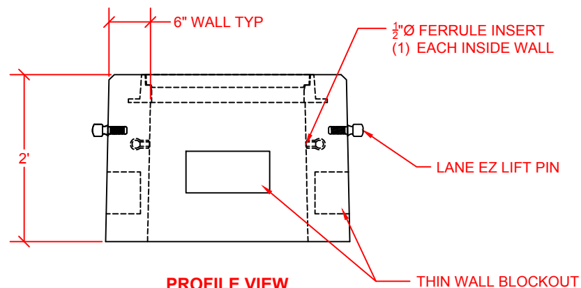
PROFILE VIEW
