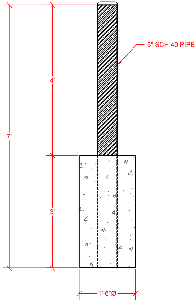
STOCK BOLLARD
