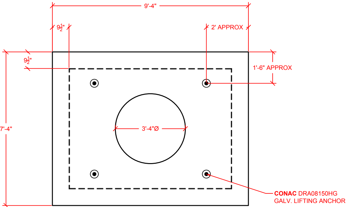
VAULT LID: PLAN WEIGHT: 6,000 LBS
