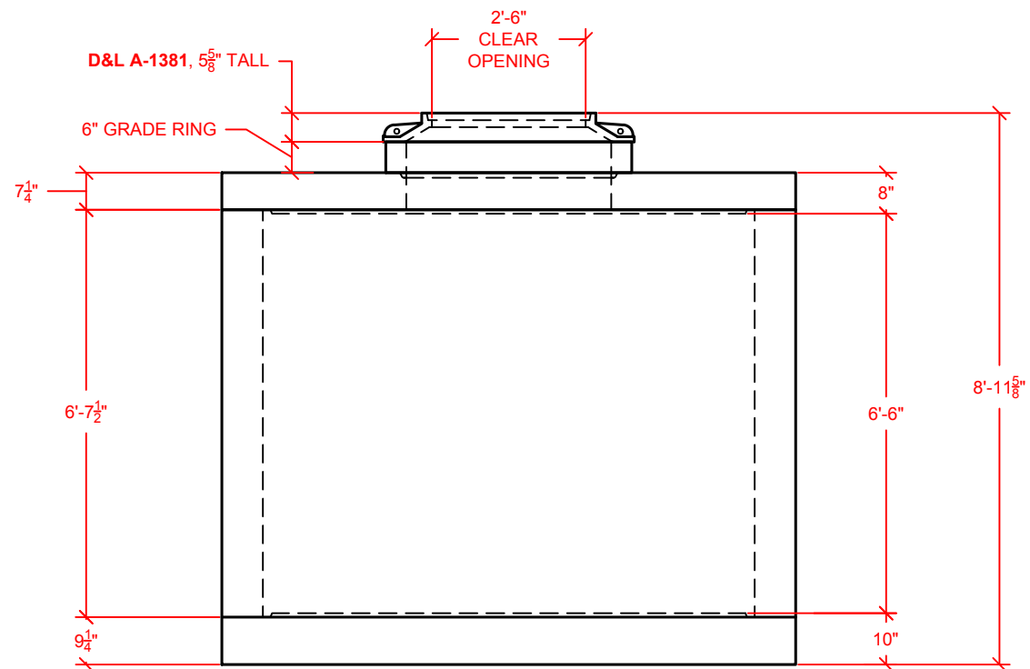
STACKED VAULT PROFILE
