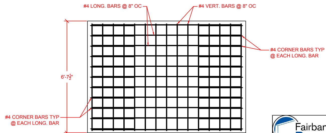
VAULT WALLS: PROFILE & REBAR LAYOUT
