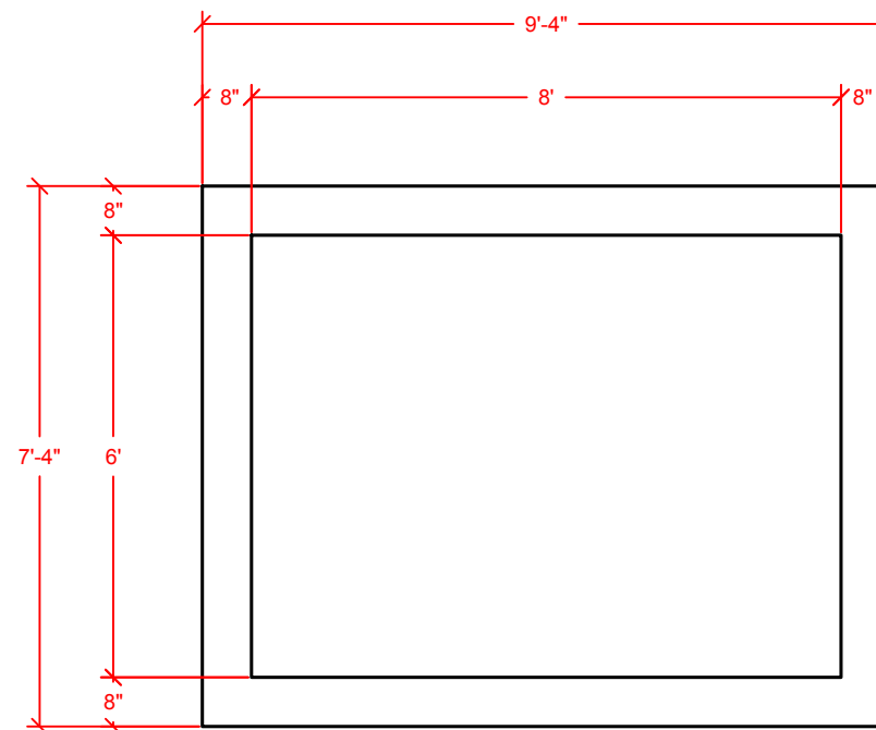
VAULT WALLS: PLAN WEIGHT: 20,000 LBS
