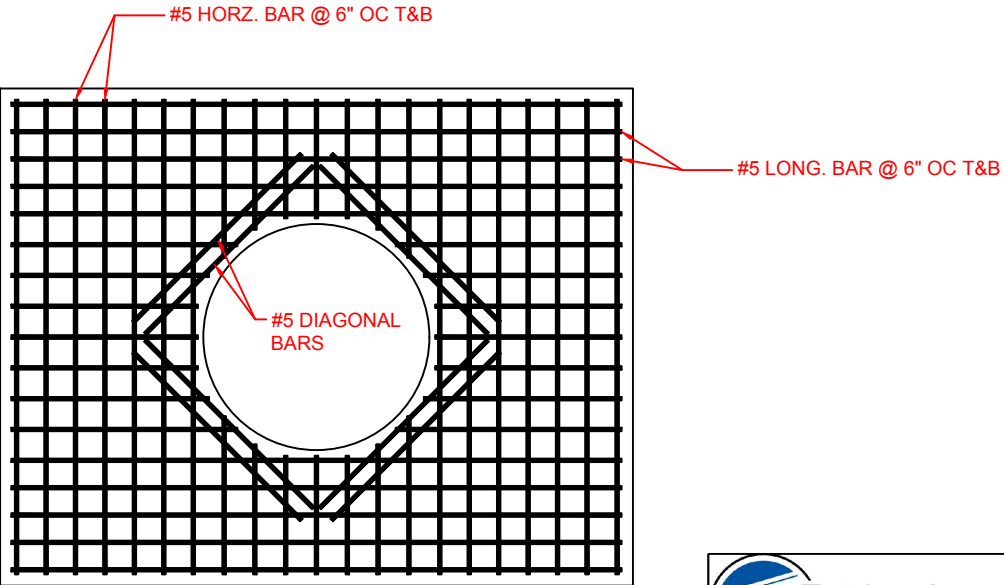
VAULT LID: REBAR LAYOUT
