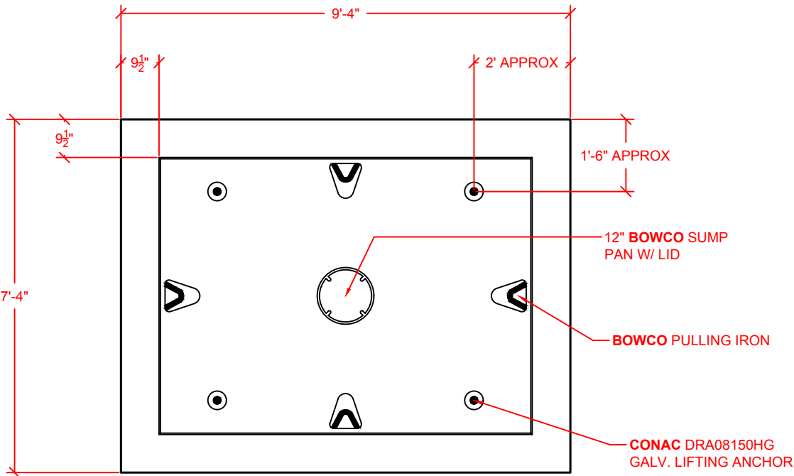
VAULT BASE: PLAN WEIGHT: 8,600 LBS
