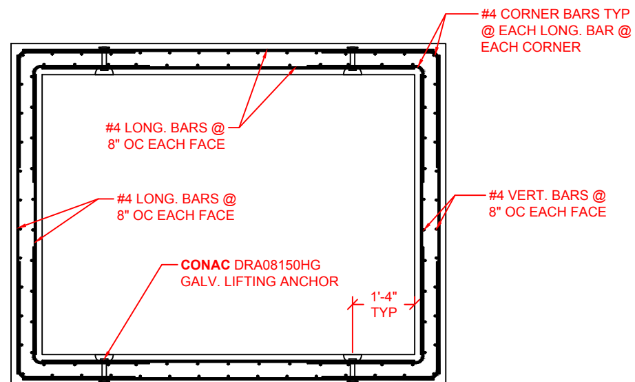
VAULT WALLS: REBAR LAYOUT
