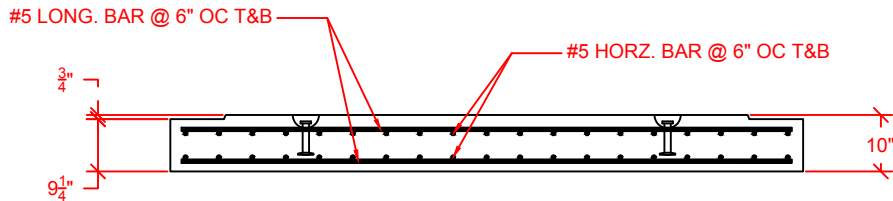
VAULT BASE: PROFILE & REBAR LAYOUT
