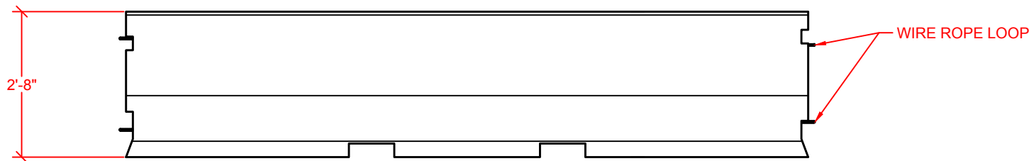
PROFILE VIEW
