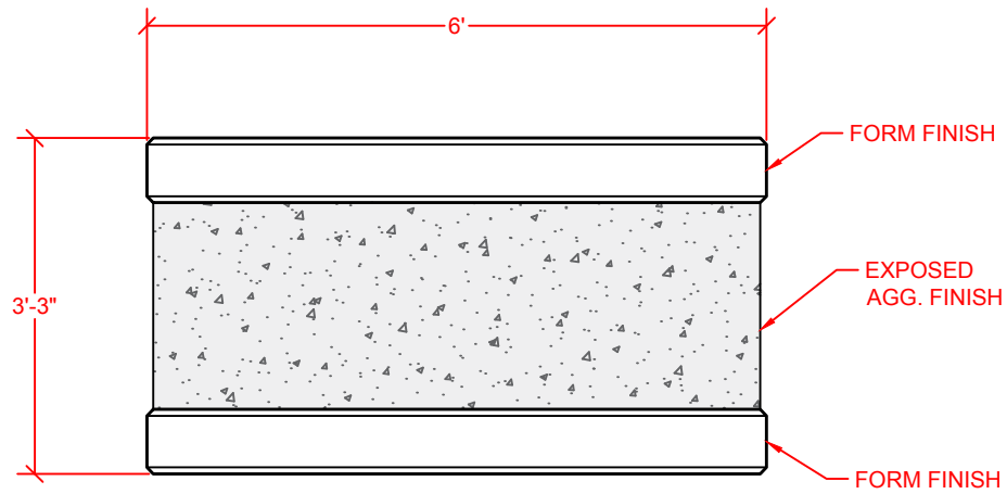
PROFILE VIEW
