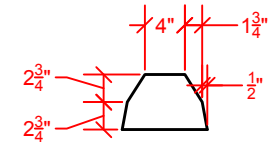
WHEELSTOP END
