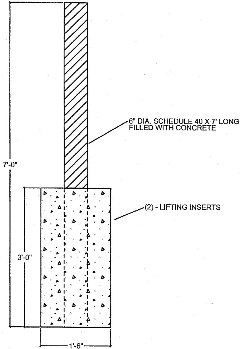
ELEVATION VIEW 7' BOLLARD
