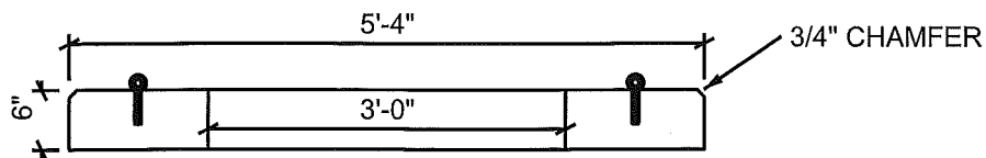
SECTION
