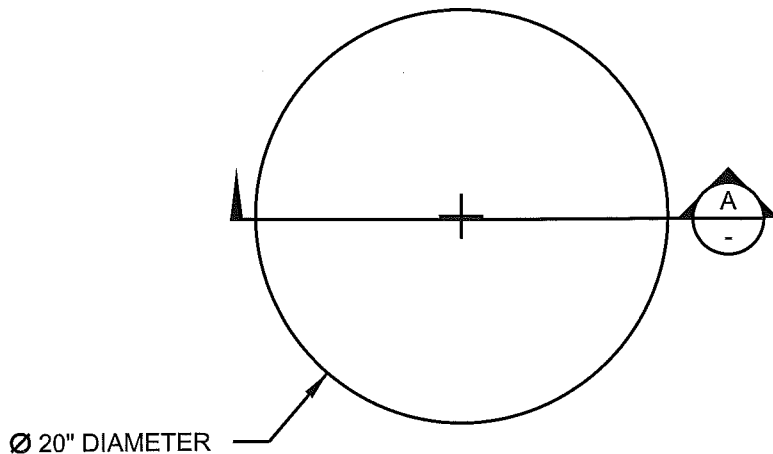
PLAN VIEW 20" ROUND PAVER
