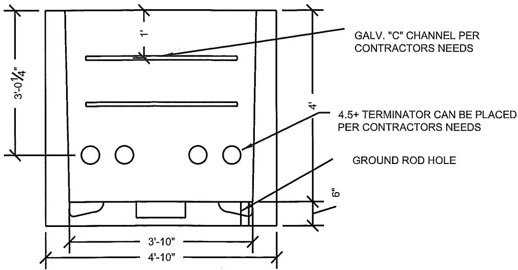
VAULT - SIDE VIEW WITHOUT LID
